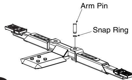
Swing Arm Superstructure
