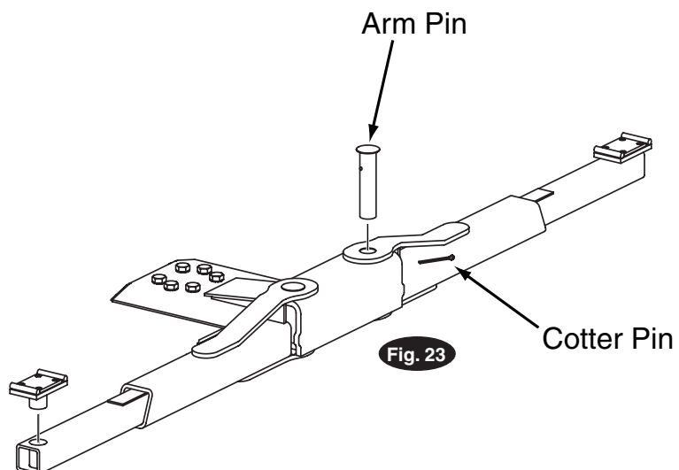
Fixed Pad Superstructure
